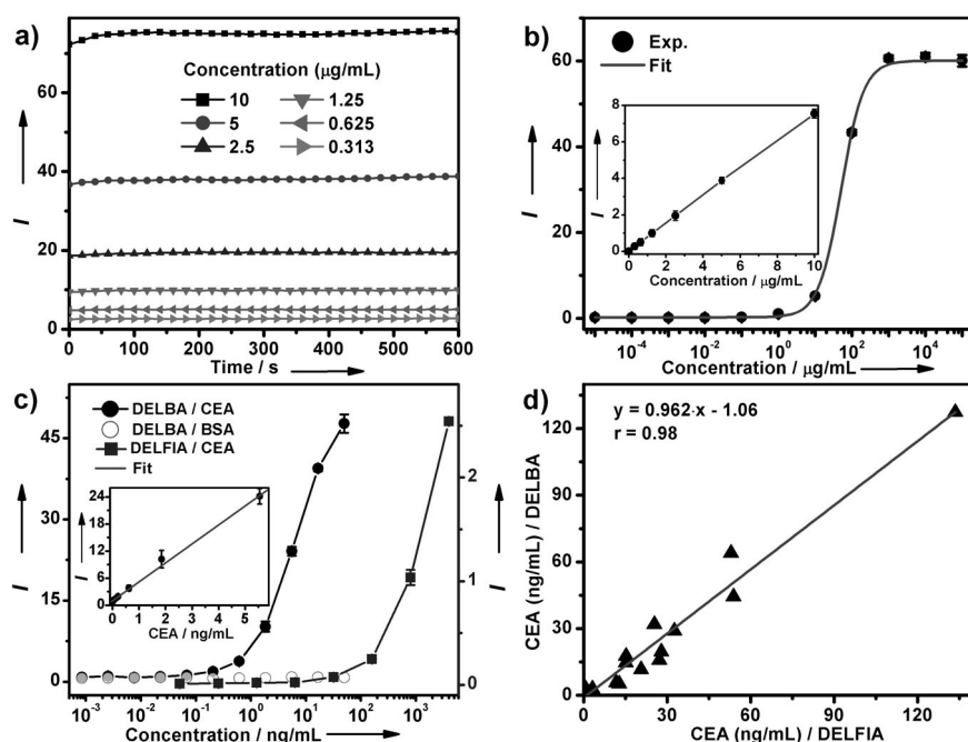
Figure 4. a) Time-dependent PL signal of ligand-free NaEuF 4 NPs at different concentrations upon addition of the enhancer solution (200 µL). b) Concentration-dependent dissolution-enhanced PL signal of NaEuF 4 NPs dissolved in the enhancer solution. Inset: the linear range of the dissolution-enhanced PL signal versus NP concentration (0–10 µg mL -1 ). c) Calibration curves for the CEA assay using DELBA (based on NaEuF 4 NPs) and the commercial DELFIA kit (based on the Eu 3+ –DTTA complex). Right-hand axis refers to DELFIA/CEA square data points. Gray circles indicate overlapped black and white circular data points. Inset: the linear range of the calibration curve for the CEA assay by DELBA. d) Correlation between DELBA and commercial DELFIA for the detection of CEA in 20 human serum samples. The axes indicate the CEA levels detected in DELBA (ordinate axis) and DELFIA (abscissa axis) experiments. b)–d) Each data point represents the mean (± standard deviation) of three independent experiments.
